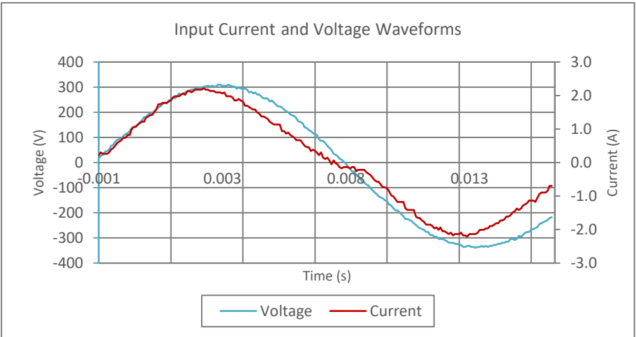
Input AC Current Waveform (ITHD = 14.16%, 50% Load)
